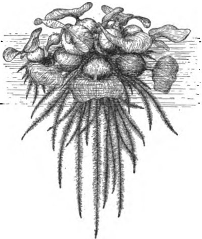
FIG. 380. — The Water Hyacinth, Eichornia crassipes ; \times \frac{1}{2} . The expanded petioles serve as floats.
